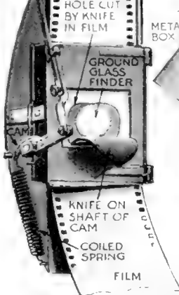
THE FILM CUTTER AND GROUND GLASS PLATE
